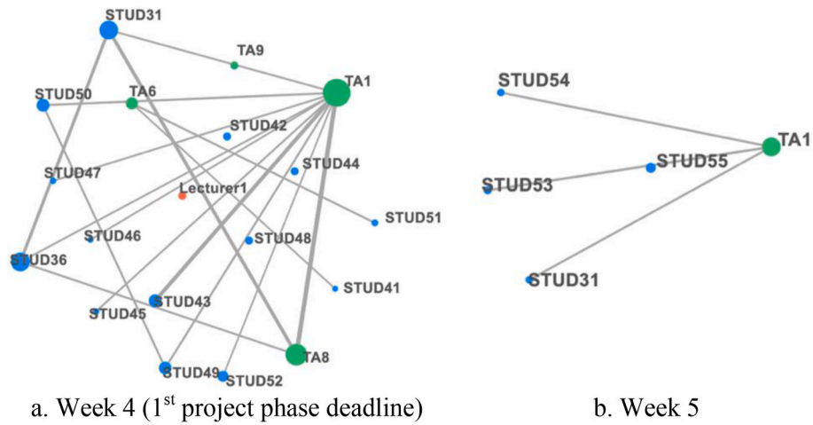
Fig. 9. Force-directed graphs for the 4th and 5th weeks of the 2018–2019 school year.
