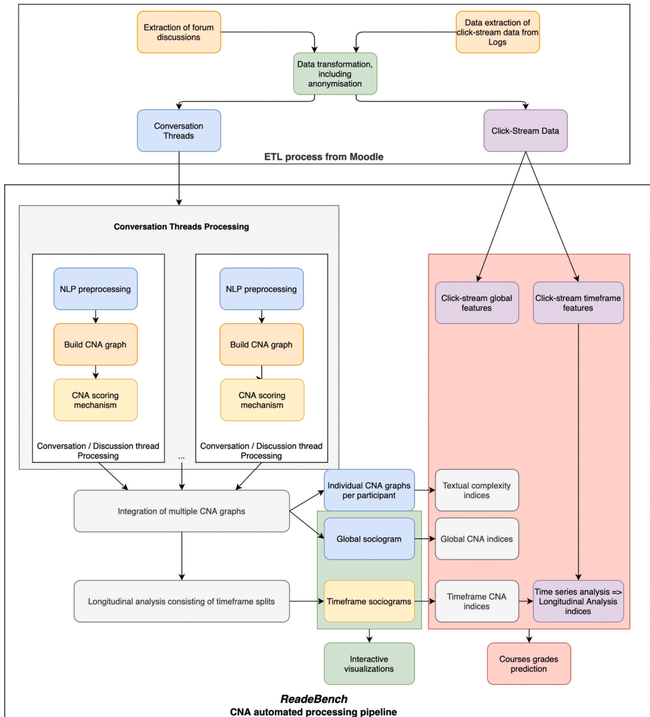
Fig. 2. ReaderBench: Processing pipeline for predicting grades and generating interactive visualizations.
