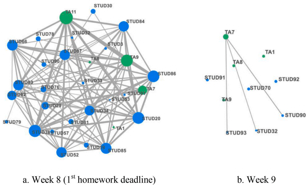
Fig. 11. Force-directed graphs for the 8th and 9th weeks of the 2019–2020 school year.
