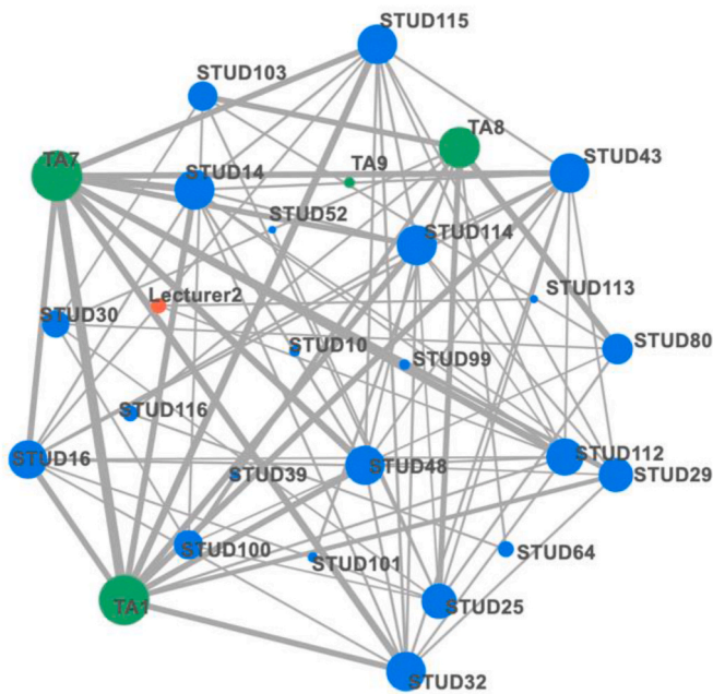
Fig. 12. Force-directed graph for the 13th week 2019–2020 school year.
