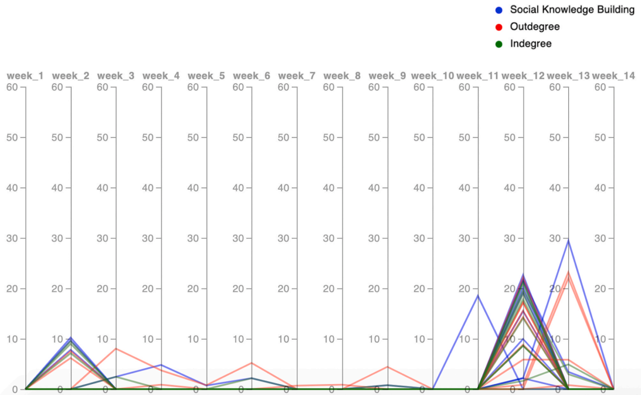
Fig. 7. Parallel view for the 10 most active students from the 2018–2019 school year illustrating trends in the community.
