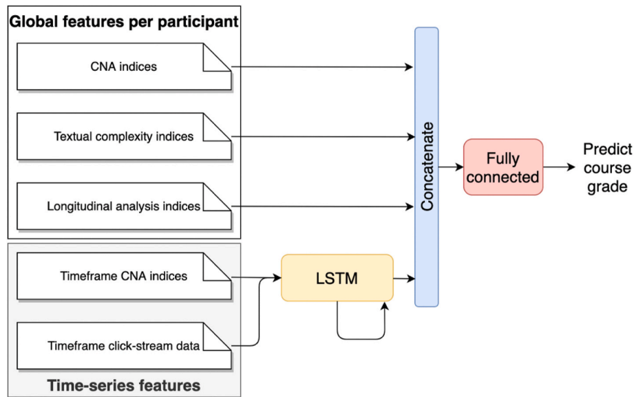
Fig. 3. RNN architecture for predicting course grades.
