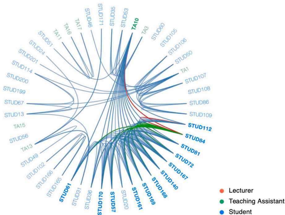
Fig. 5. Hierarchical edge bundling view for the 13th week 2018–2019 school year.
