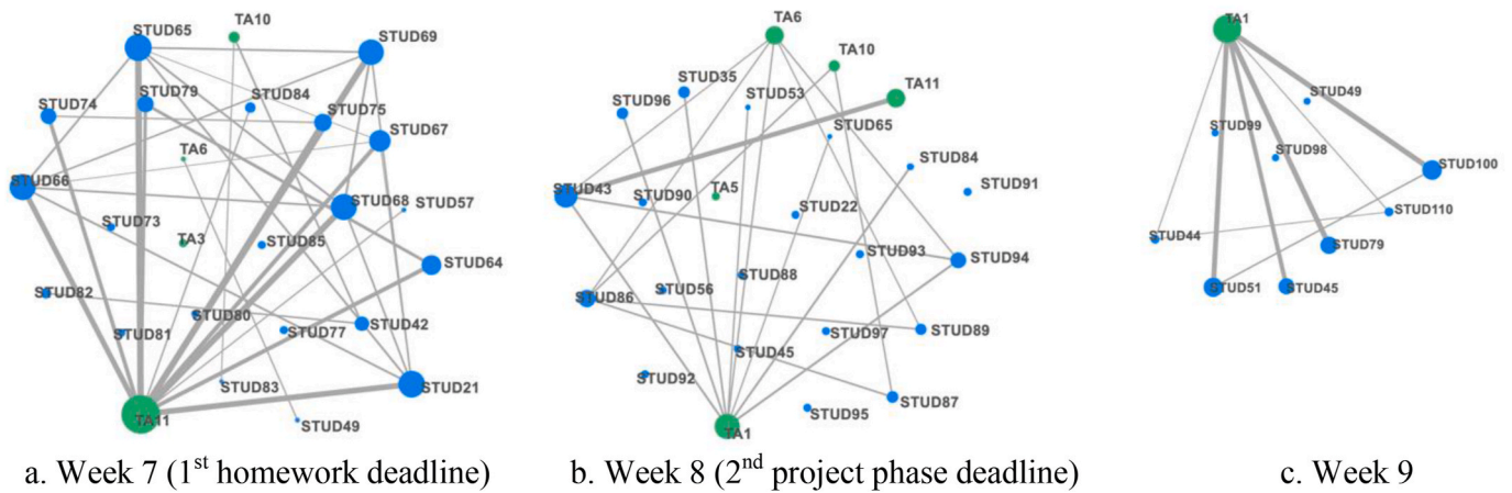
Fig. 10. Force-directed graphs for the 7th, 8th and 9th weeks of the 2018–2019 school year.
